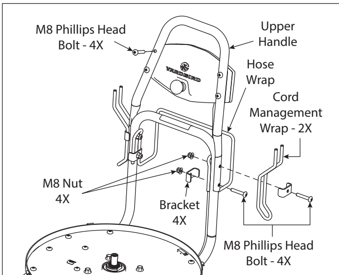
Figure 5 - Steps 10-12
